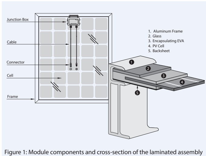
Figure 1: Module components and cross-section of the laminated assembly
